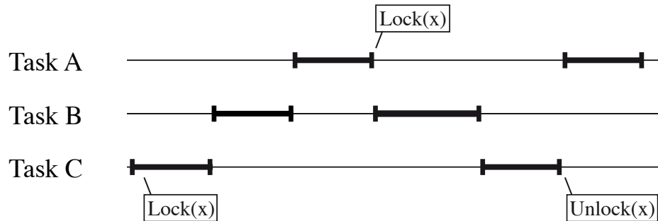
Figure 10.4: Priority Inversion
