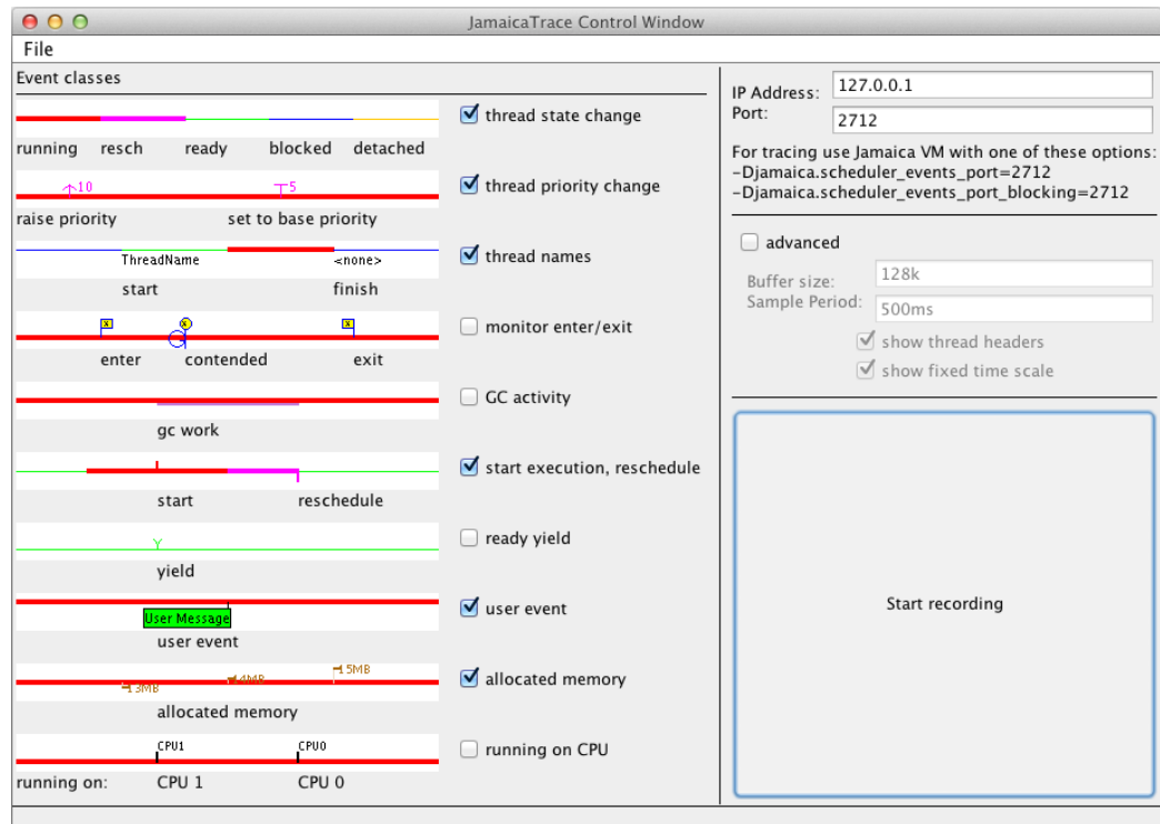
Figure 17.1: Control view of JamaicaTrace
