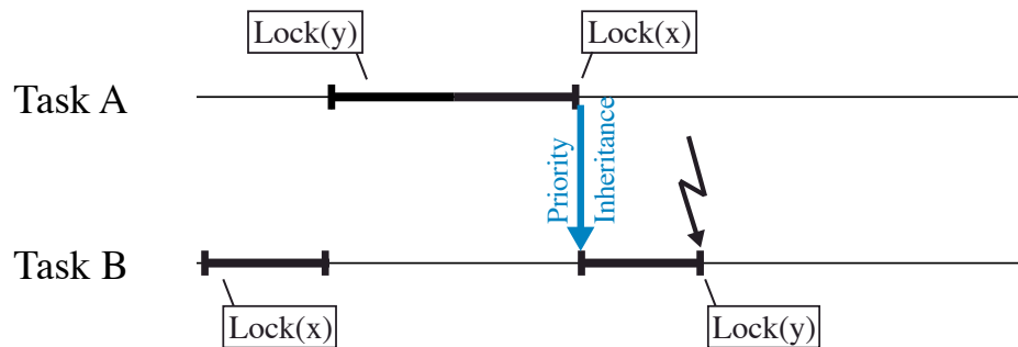
Figure 10.7: Deadlocks are possible with Priority Inheritance
