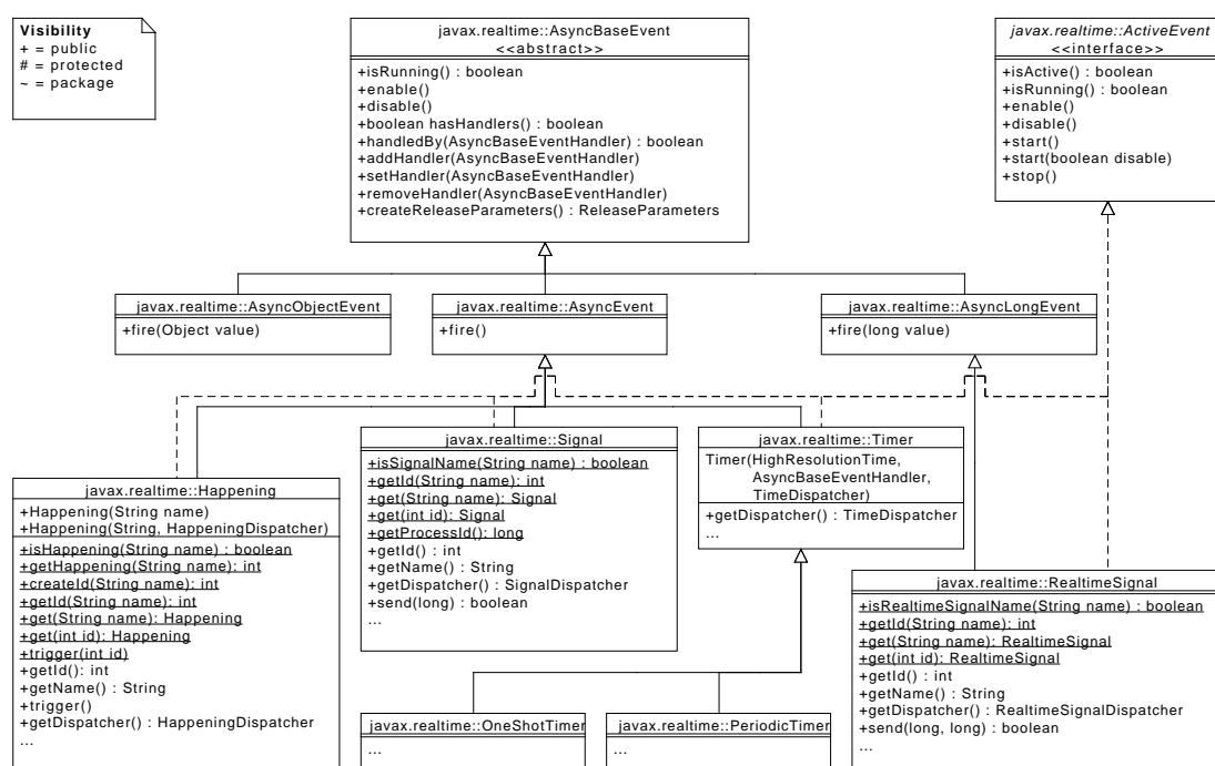
Figure 8.1: The Event Class Hierarchy
