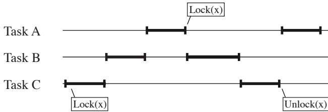
Figure 9.4: Priority Inversion
