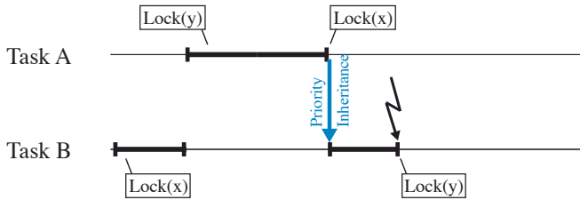
Figure 9.7: Deadlocks are possible with Priority Inheritance
