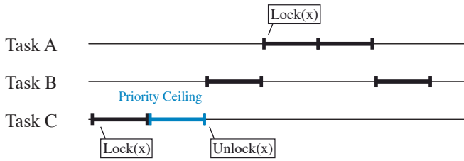
Figure 9.6: Priority Ceiling Emulation Protocol
