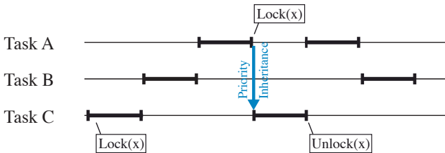
Figure 9.5: Priority Inheritance
